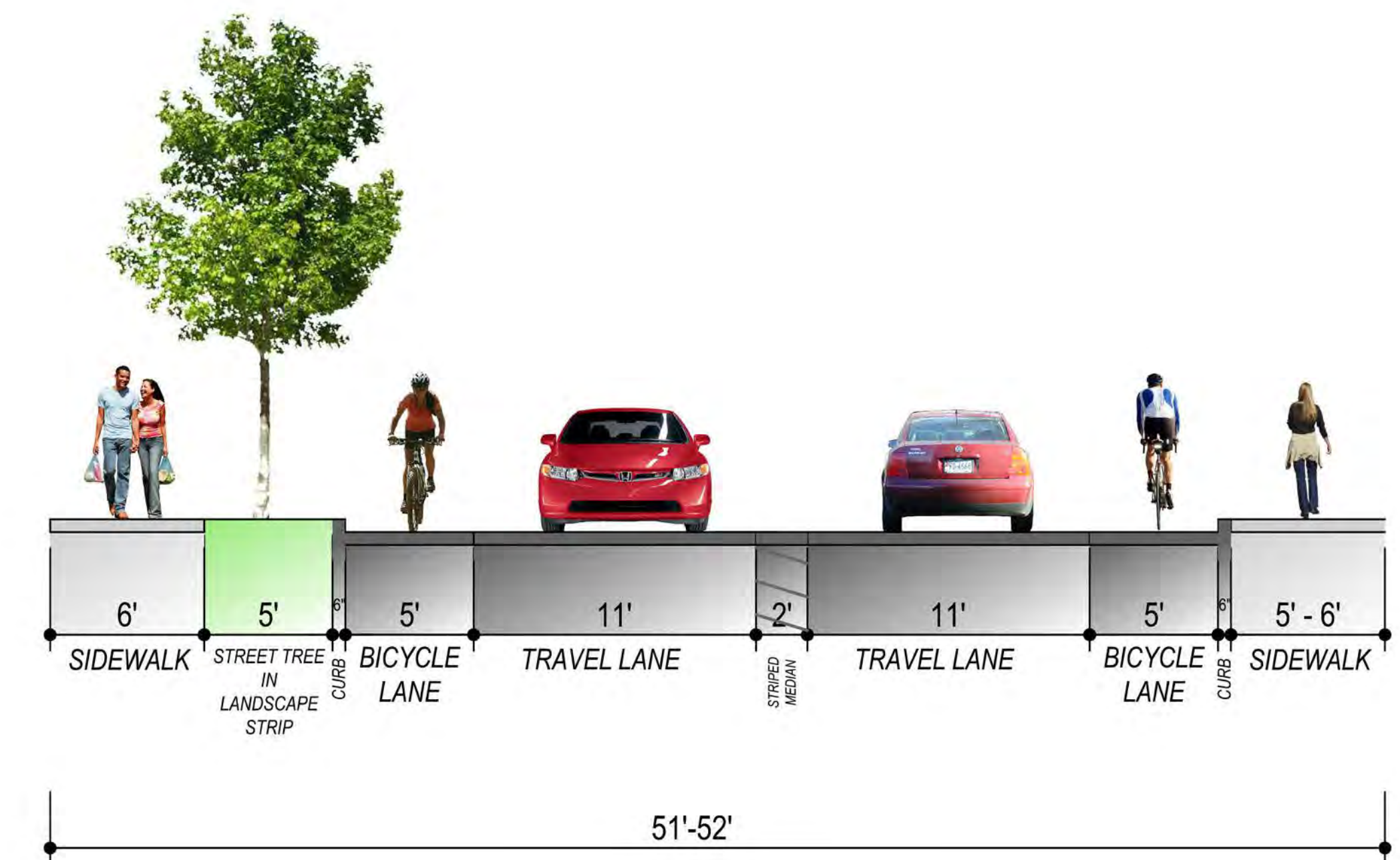
SECTION D - EAST HIGH ST. BETWEEN 9 1/2 ST. AND CFA
