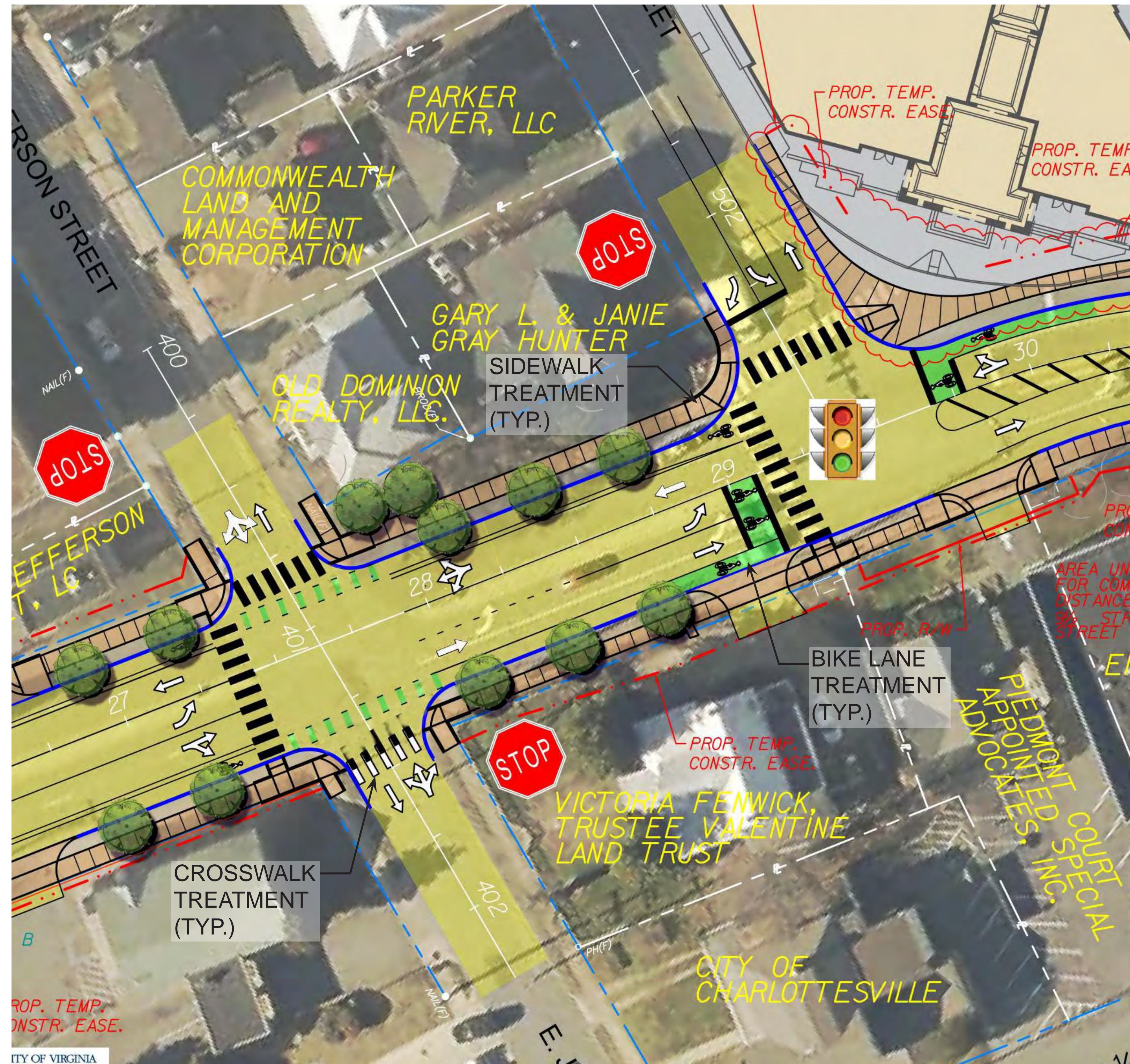
Standard Asphalt Crosswalks: Striped / Painted
